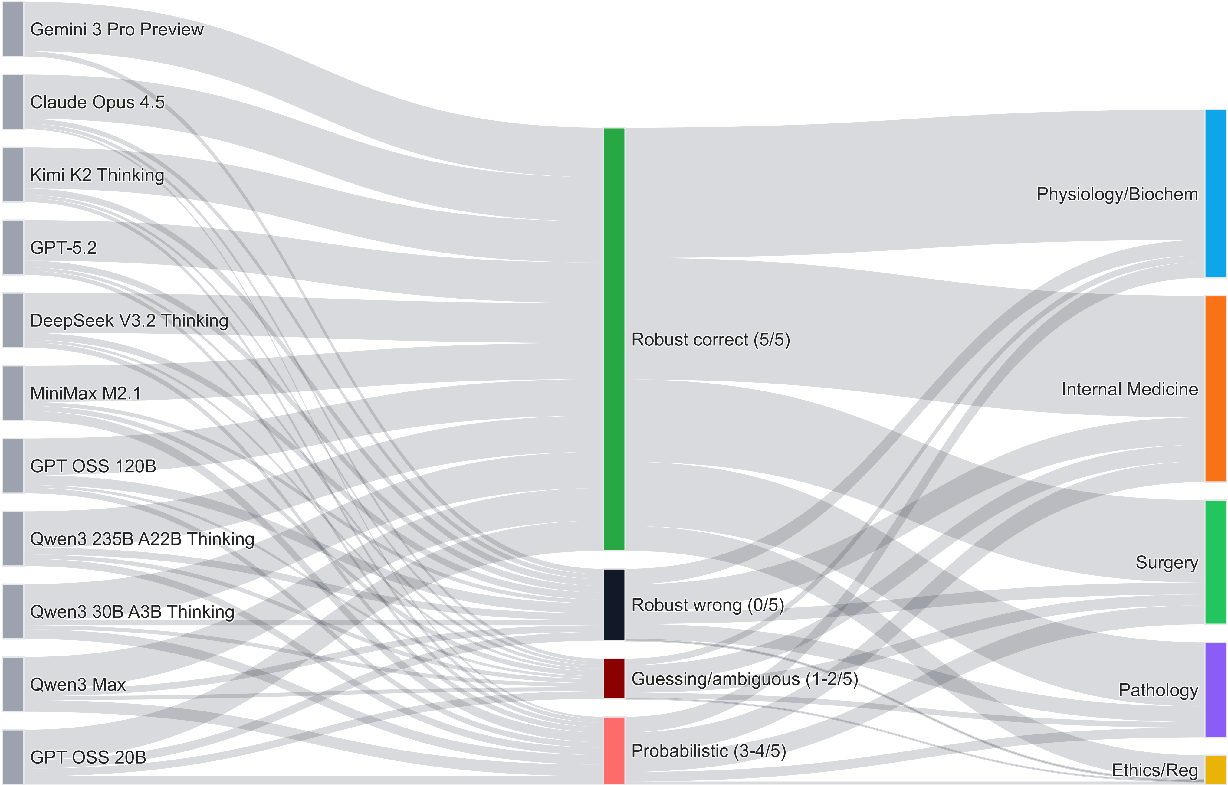
Agentic: Consistency Sankey (model -> consistency -> discipline)
