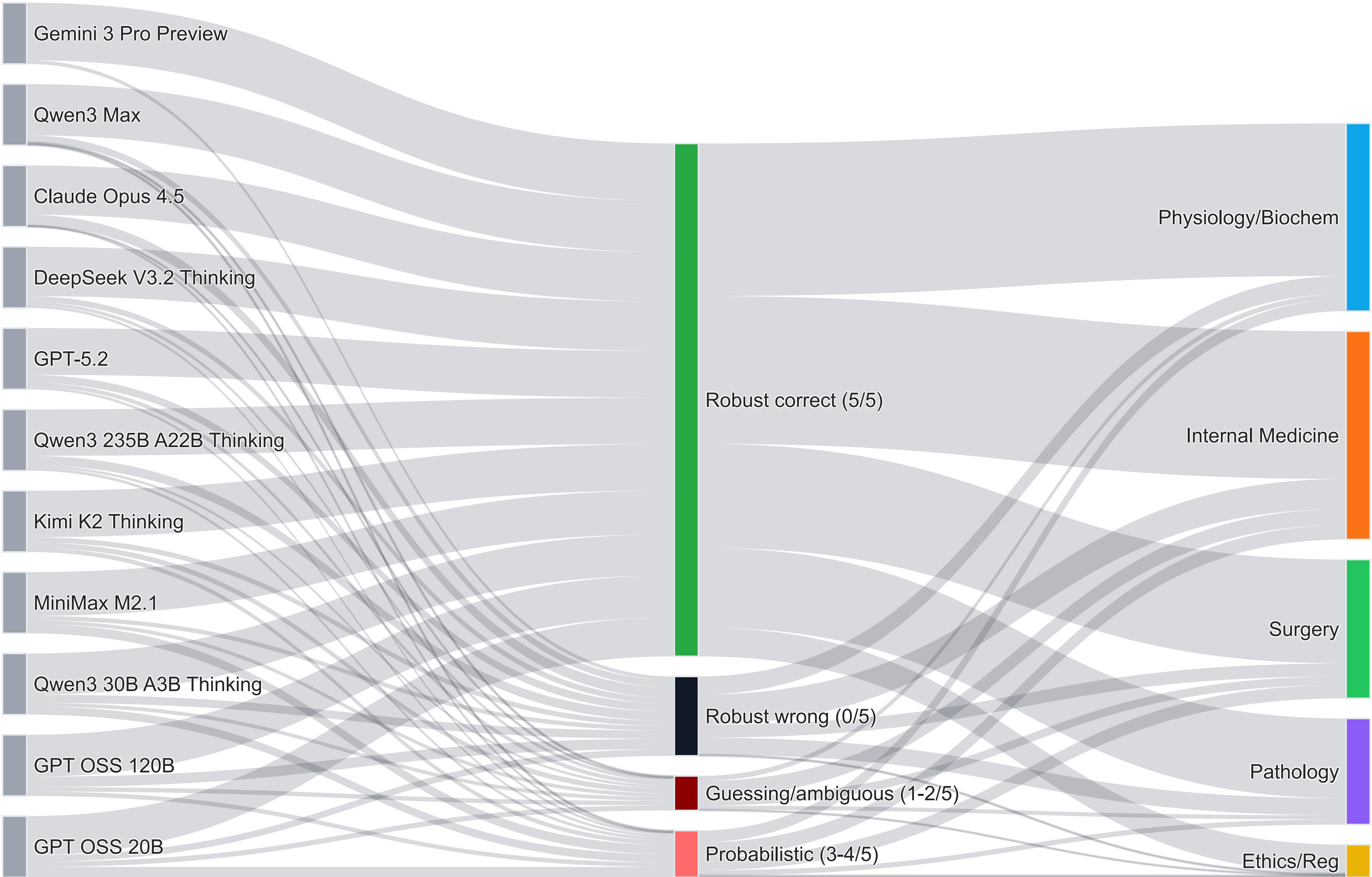
Baseline: Consistency Sankey (model -> consistency -> discipline)
